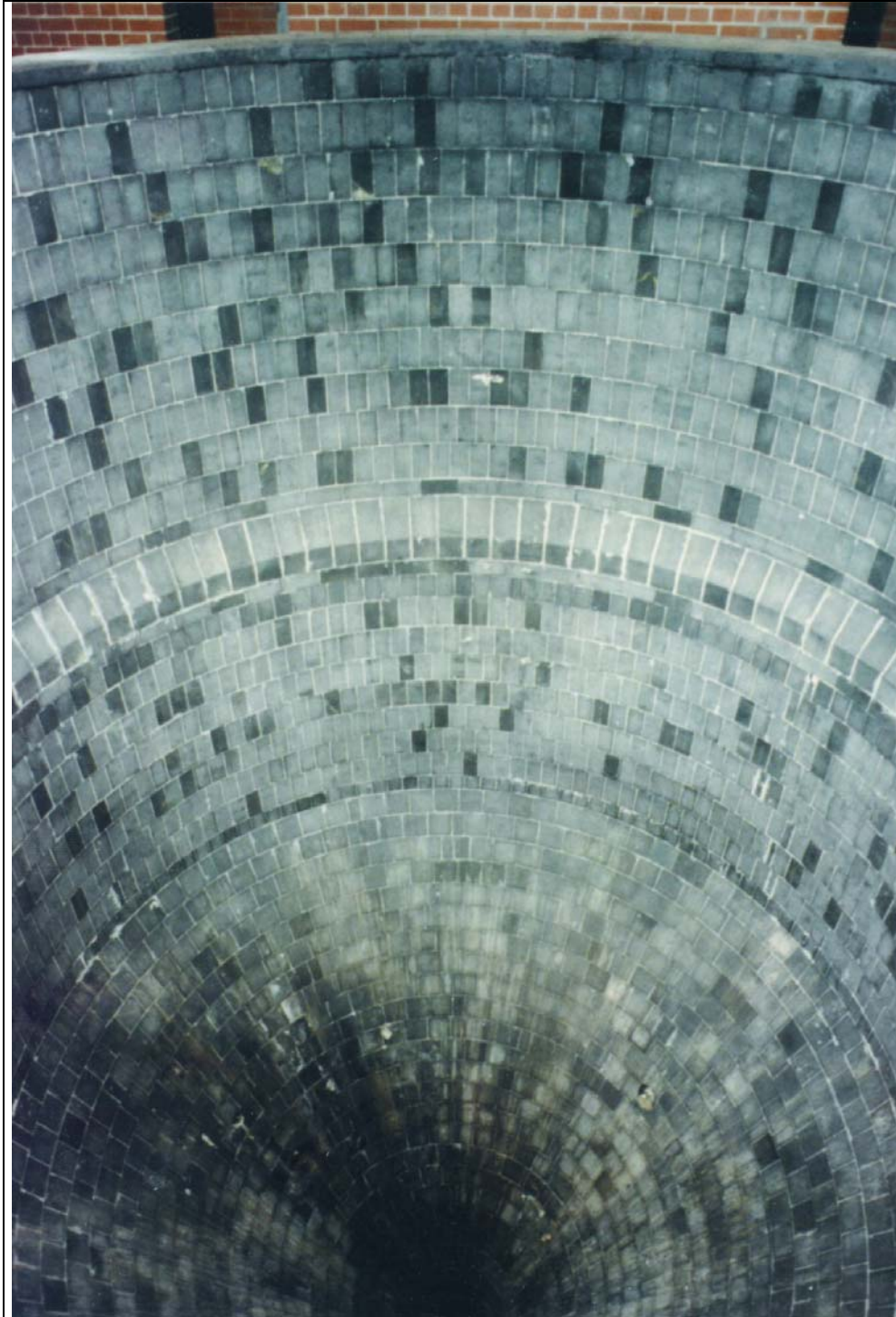
Attack tank with Carbon- Bricks in the Face course, H 2 SO 4 - Process
